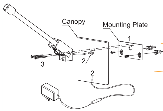
Wand Light Exploded Diagram
